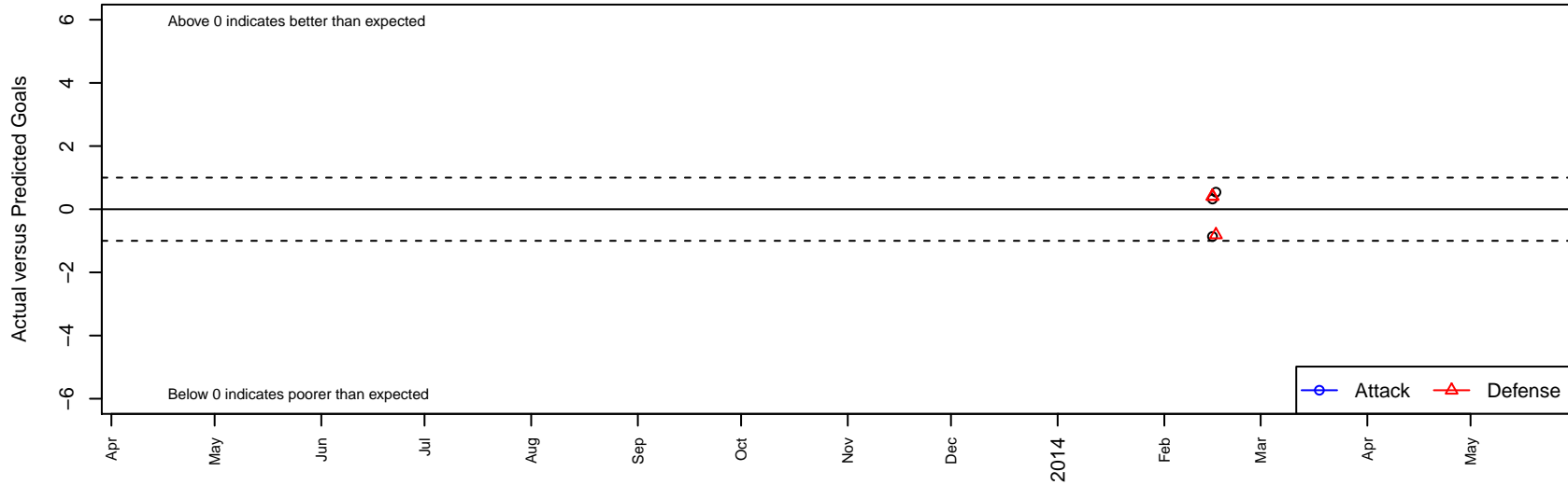
TSA Red B00 Dots are actual minus expected GF (blue circles) and GA (red triangles). Blue line is smoothed change in attack strength. Red is smoothed change in defense strength.
